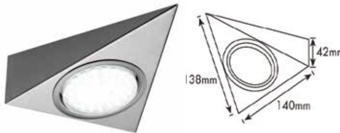
SE11147SS with SE10156CW lamp
