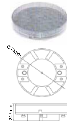
SE10156 - GX53 LED Lamp
